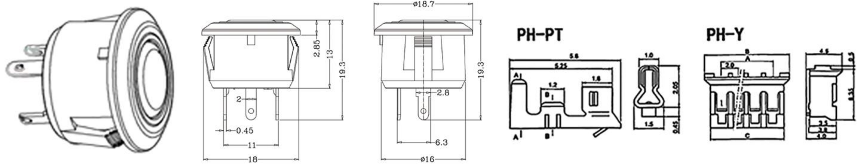
大触摸头/塑料款(可选金属头) Large Touch Head/Plastic(Or Metal)
