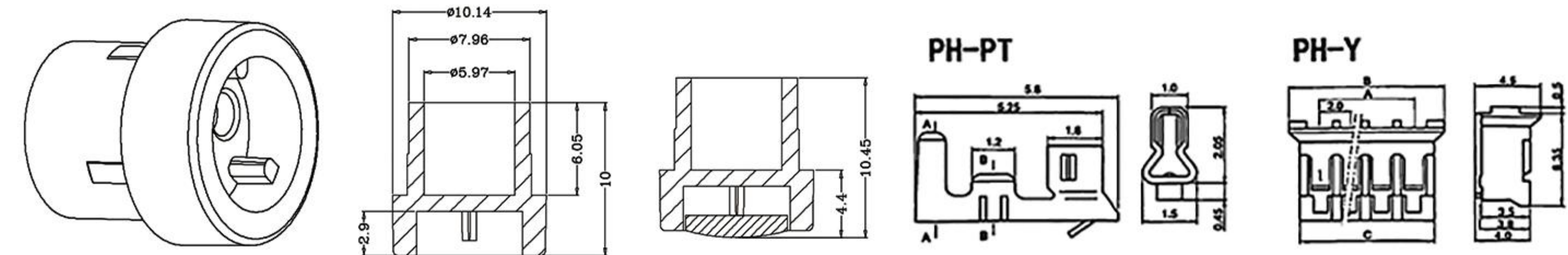
小触摸头/塑料款 Small Touch Head/Plastic Version
